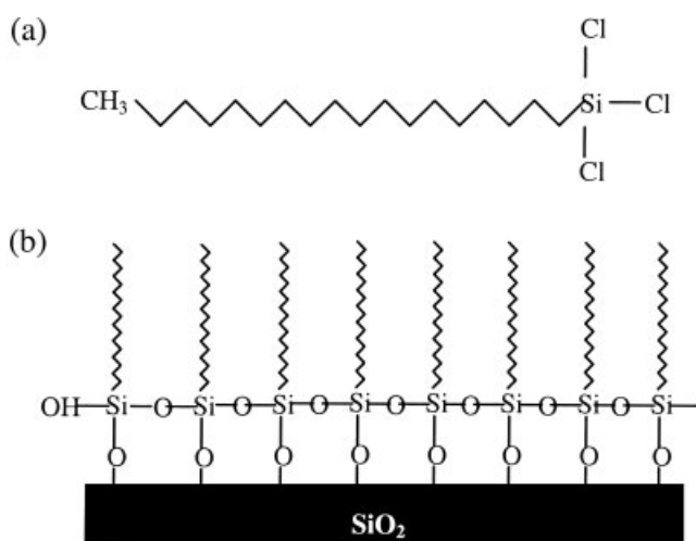
Figure 1. (a) Structure of octadecyltrichlorosilane (C 18 ). (b) Possible structures of C 18 monolayer on the SiO 2 surface. (Drawing is not to scale.)
