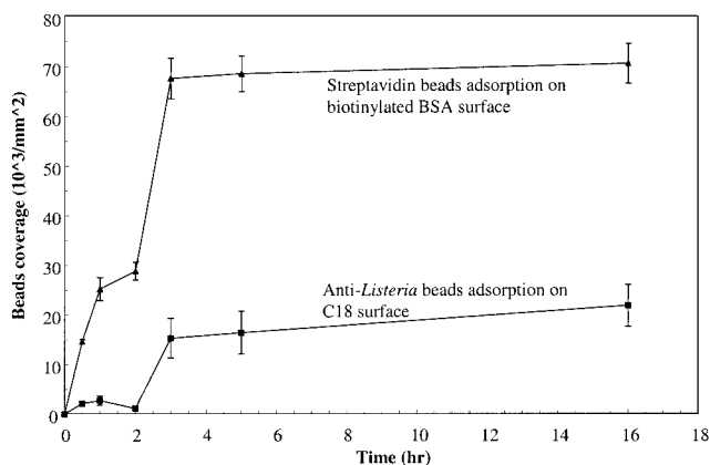
Figure 4. Adsorption kinetics of streptavidin microbeads on a C 18 surface pre-adsorbed with biotinylated BSA and of anti- Listeria antibody-coated microbeads on a bare C 18 surface. (Error bar represents one standard deviation in 10 3 beads/mm 2 using data in triplicate.)
